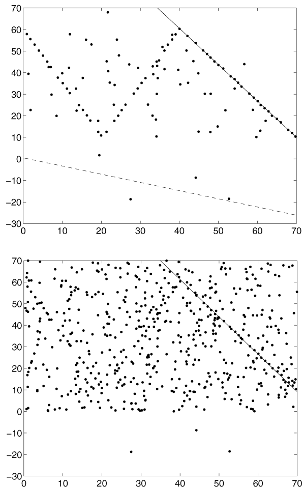
Fig. 2. Top: Line fitting to data scanned from Fig. 9 of [1]. The solid line was obtained with the KA-algorithm [2] in our laboratory. The dashed line is the result attributed to the KA-algorithm in Fig. 10 of [1]. Bottom: The fitting obtained with the KA-algorithm is stable even in the presence of additional outliers.
