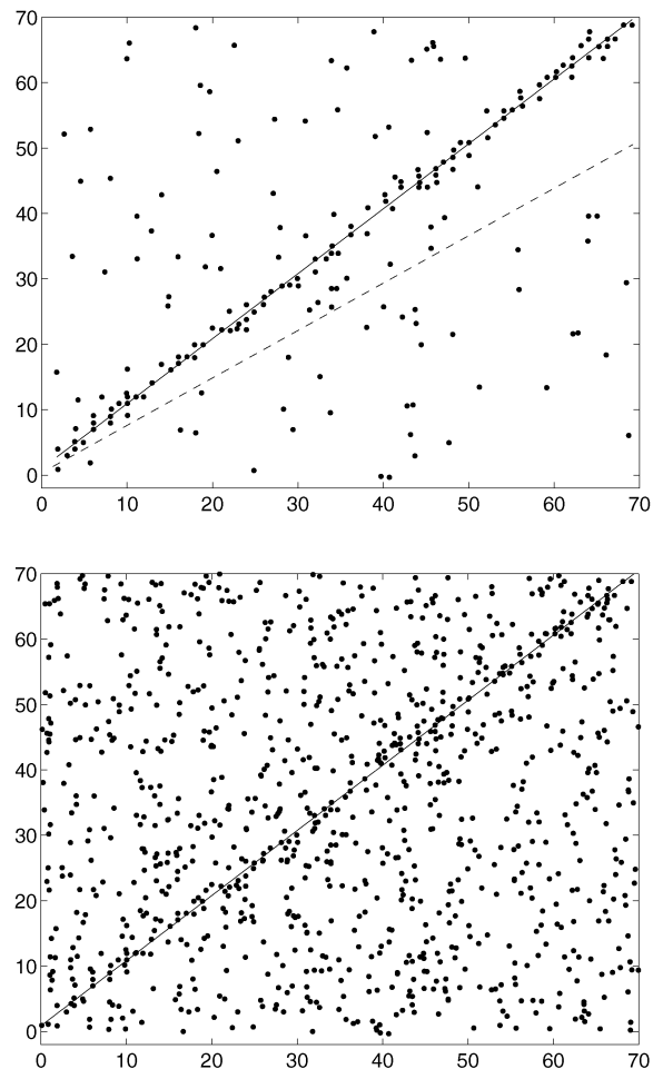
Fig. 1. Top: Fitting a line to a set of data points taken from Fig. 3 of [1]. The solid line was obtained in our laboratory using the KA-algorithm [2]. The dashed line is the result attributed to the KA-algorithm in Fig. 6 of [1]. Bottom: The fitting quality obtained with the KA-algorithm remains high even when the number of outliers is increased.
